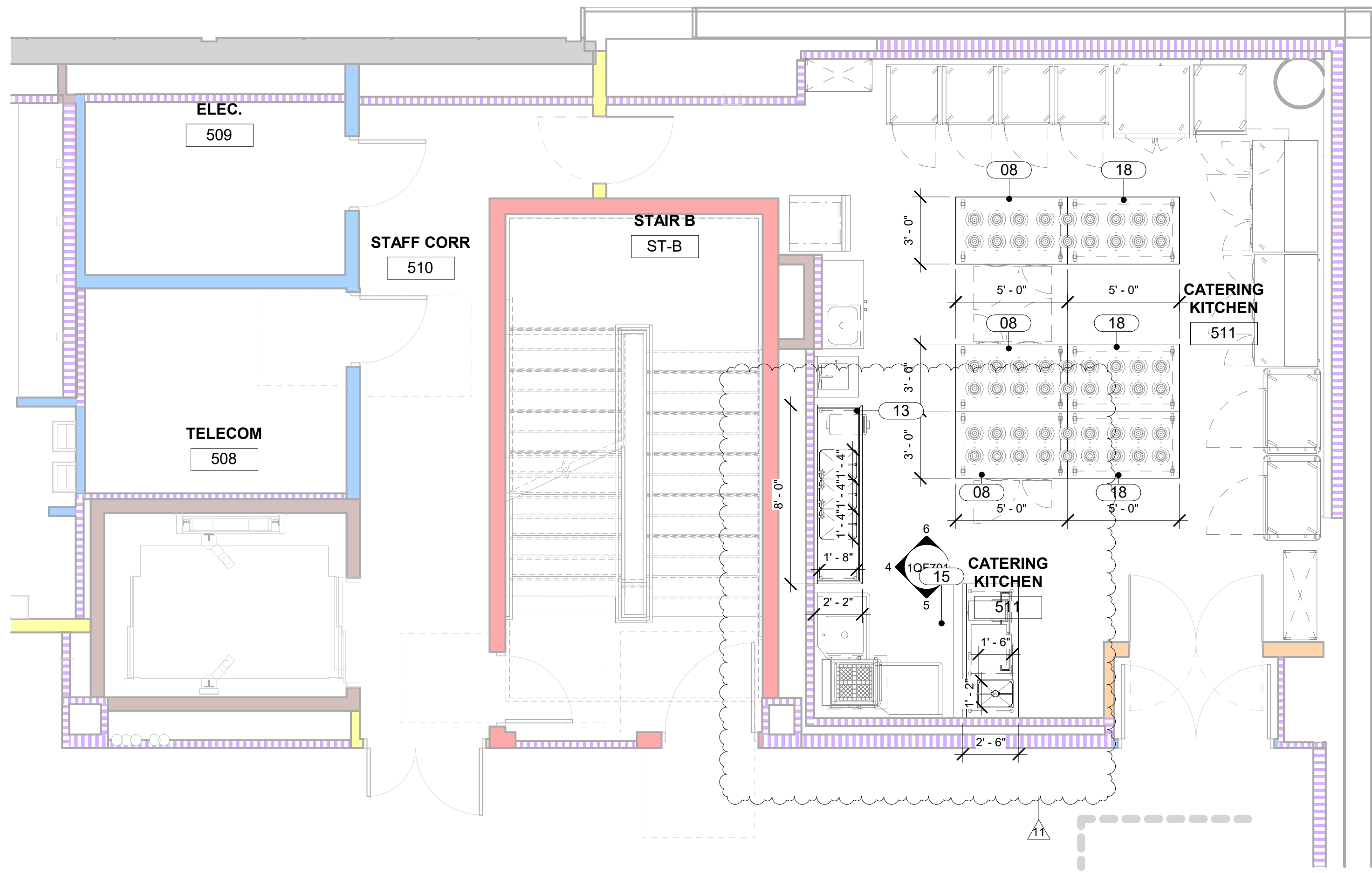
1 FOODSERVICE CUSTOM FABRICATION PLAN - CATERING 1/4" = 1'-0"
